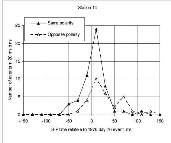
Fig. 1. An example of distribution of S-P times relative to the reference event of 1976 day 76. Events of polarity same as and opposite to the reference event are plotted separately.
