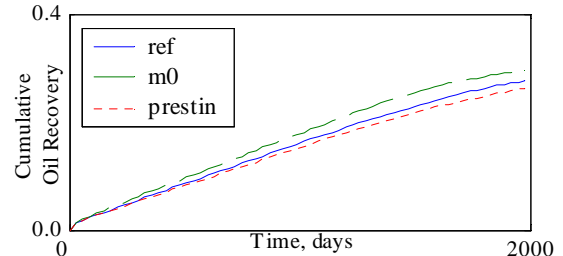
Figure 4. Comparison of dynamic results. Plot of cumulative oil recovery as a function of time for (a) the true or reference case (ref), (b) mean of initial models (m0), and (c) mean of proposed inversion algorithm (prestin).
