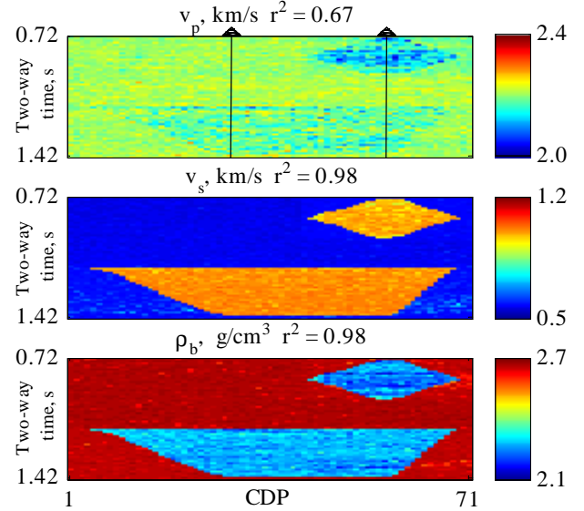
Figure 2. Cross-sections of the mean of inverted compressional-, shear-wave velocities, and bulk density for ten independent realizations obtained with the proposed inversion algorithm. Global correlation coefficients ( r^2 ) are calculated with respect to the reference model of elastic properties.
